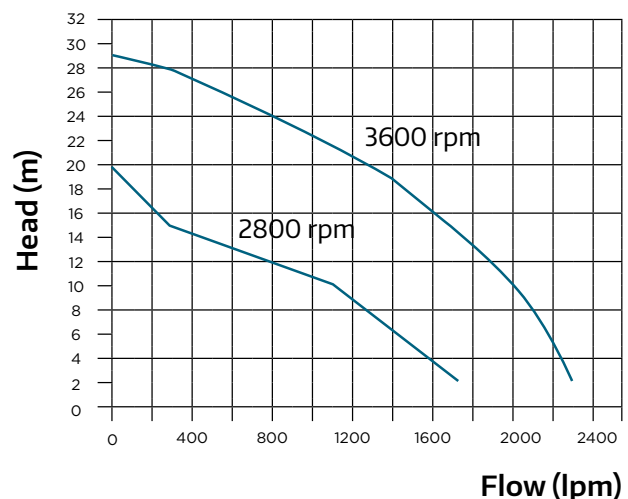
TrashLib – 4" L
