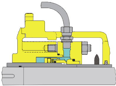
uncooled, balanced
