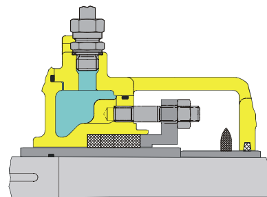
with jacket-cooling
