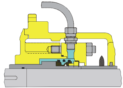
uncooled, unbalanced
