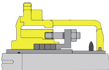
uncooled
