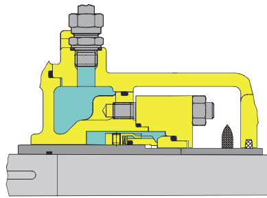
cooled, balanced
